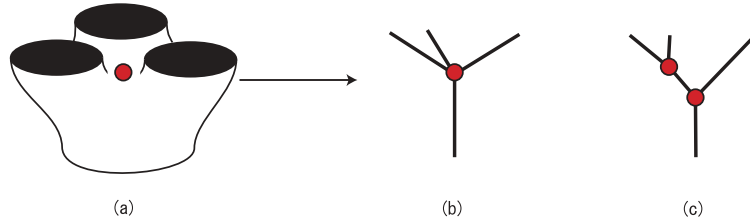
Fig. 5. An example of a degenerate singular point (a) where the singular point connects three contours to one contour (b) which can also be interpreted as the combination of two 2-to-1 singular points that coincide at this point (c)
